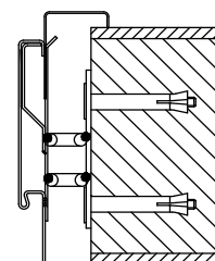
Type D2 Weld with plug/screw fitting Applicable for VarioFrame
