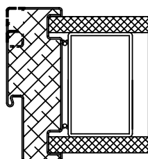
Type E Installation onto the gypsum board of steel grid
