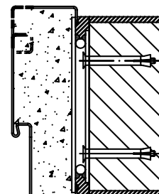
Enclosed wall frame connection
