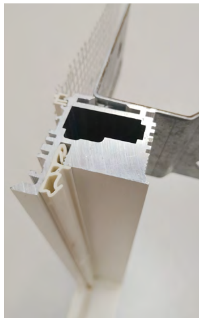
Profile and accessories of hidden frame
