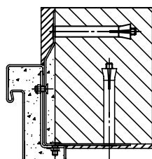
Corner frame connection
