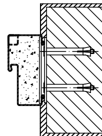
Type D2 Weld with plug/screw fitting
